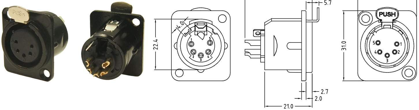
FC61950 - FEMALE XLR 5DCF/BM BLACK WITH LATCH
