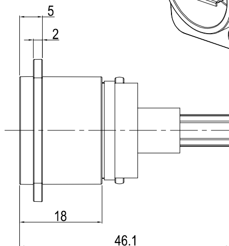
CP30117 - FT XLR FIREWIRE IEEE 1394 METAL
