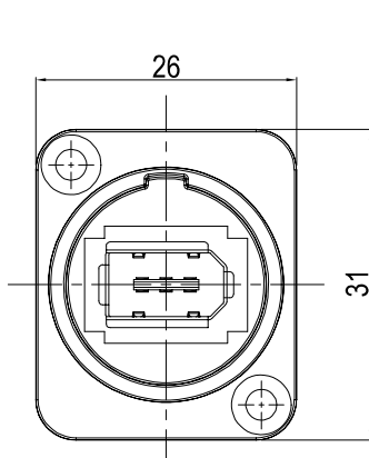
CP30117 - FT XLR FIREWIRE IEEE 1394 METAL
