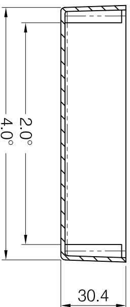
SECTION B-B
