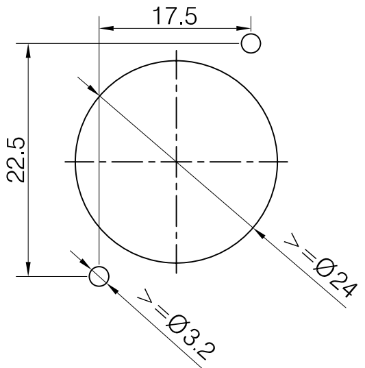
FIXING HOLE DETAIL (SELF-TAPE SCREW FIXING)
