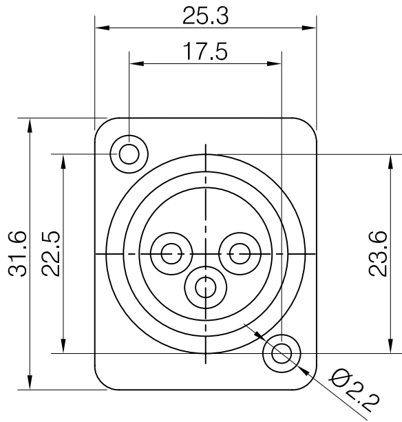
FIXING HOLE DETAIL (SELF-TAPE SCREW FIXING)
