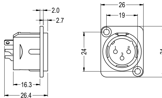
FC61905 - XLR SOCKET MALE 3DCM/BM Scale 2x1
